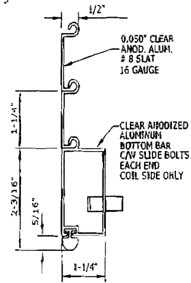
SECTION THRU BTM. OF CURTAIN SCALE: 1/2" = 1'
