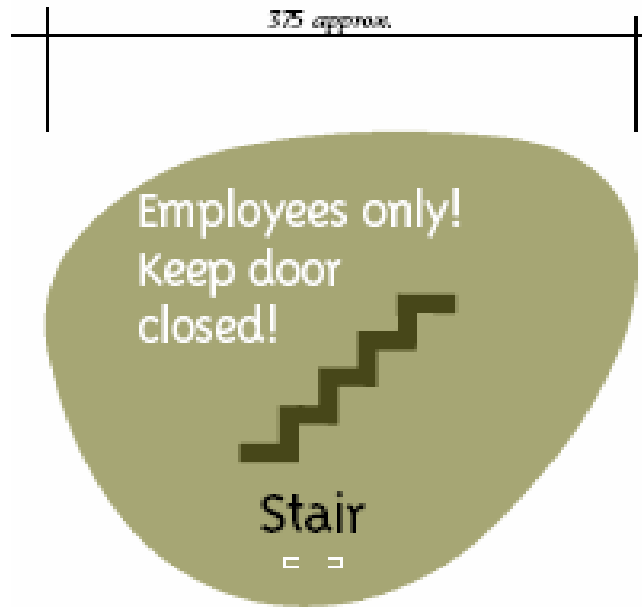
S.2 Stair ID – submit 1/2 size per plot 375mm wide 25mm (cap) tactile legend; braille
